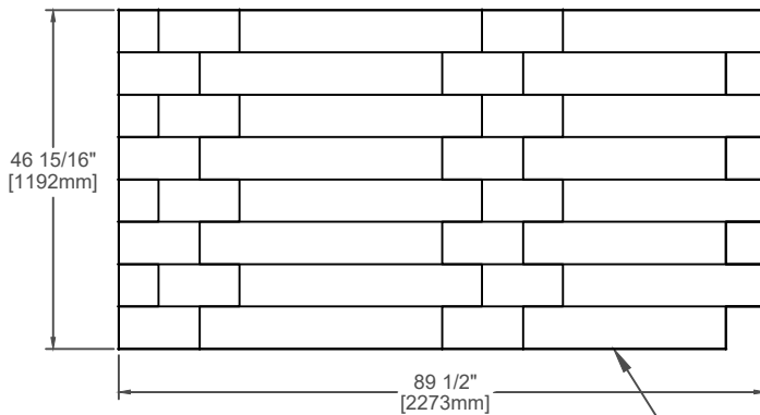
610STWV-1 ONE SIDED INTERLOCKING SHEET
