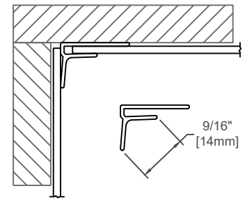
INSIDE CORNER
