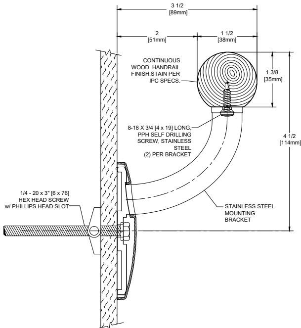
MOLDED BRACKET SECTION VIEW
