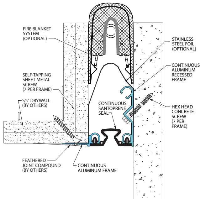
Fire Blanket System (114-A09-050 system shown)
